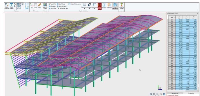
Physical modeling capabilities enable engineers to improve participation in BIM workflows, automatically generating the analysis models for both simple and complex structural analysis.
